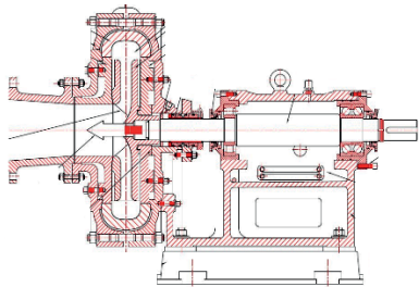
Horizontal MP Slurry Hard Metal & Rubber Lined Double Case Design C/W Dry Gland Expeller / Mechanical Seals
